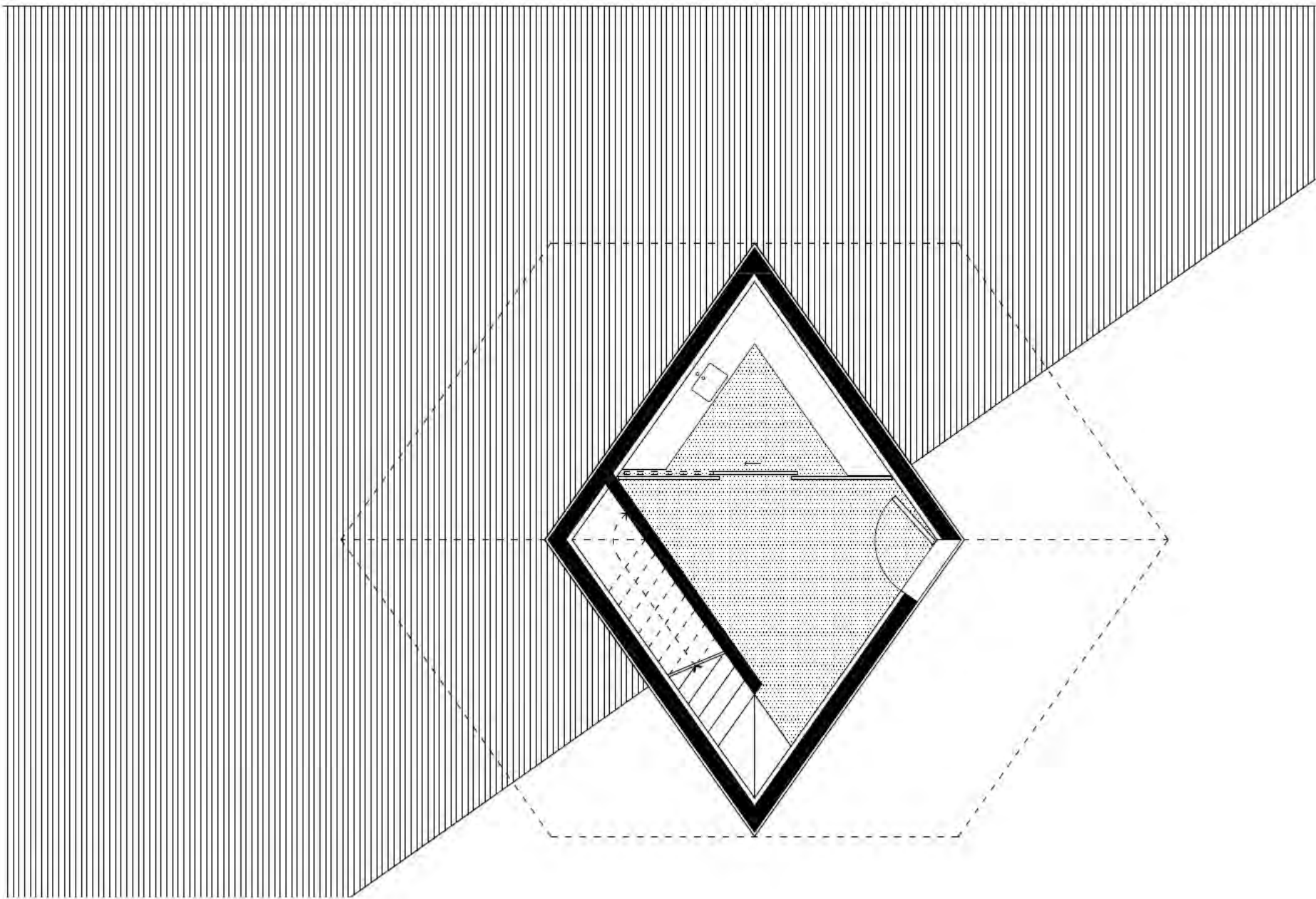
PIANTA DEL PIANO TERRA/GROUND FLOOR PLAN
